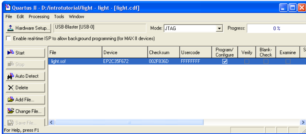
Figure 42. The updated Programmer window.
