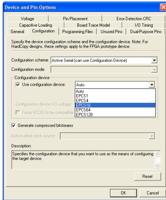
Figure 45. Specifying the configuration device.
