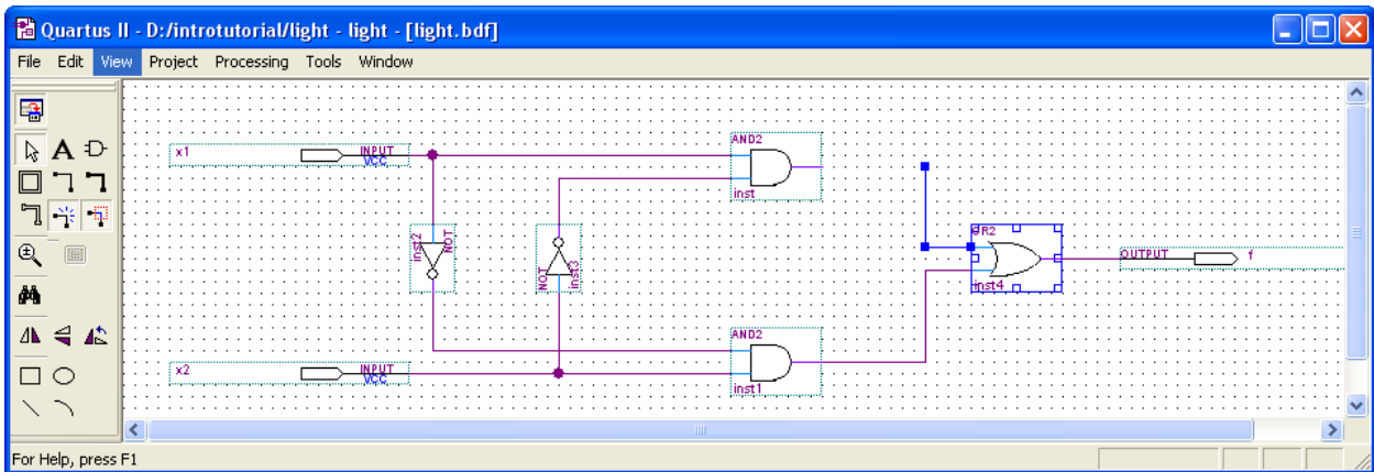
Figure 23. Identifying the location of the error.
