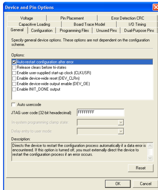
Figure 44. The Options window.
