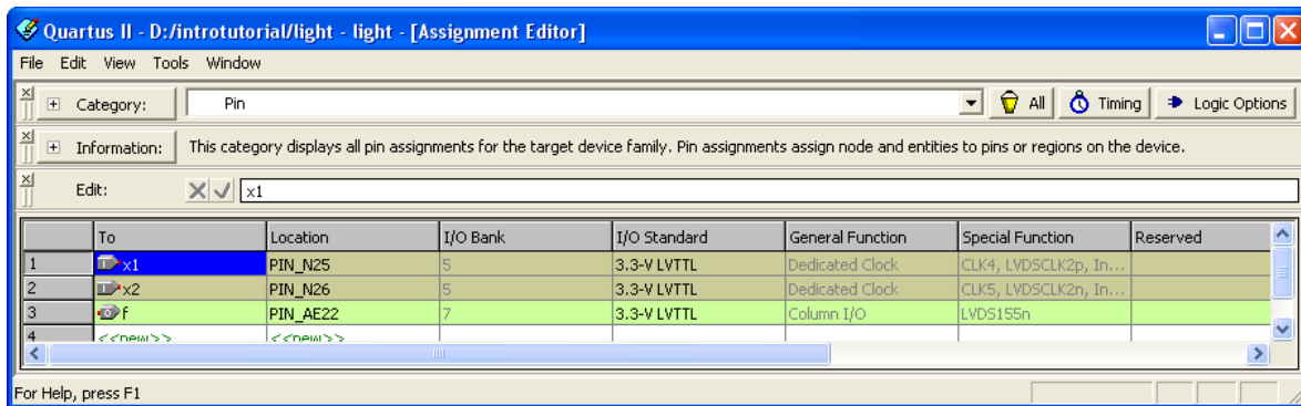
Figure 27. The complete assignment.
