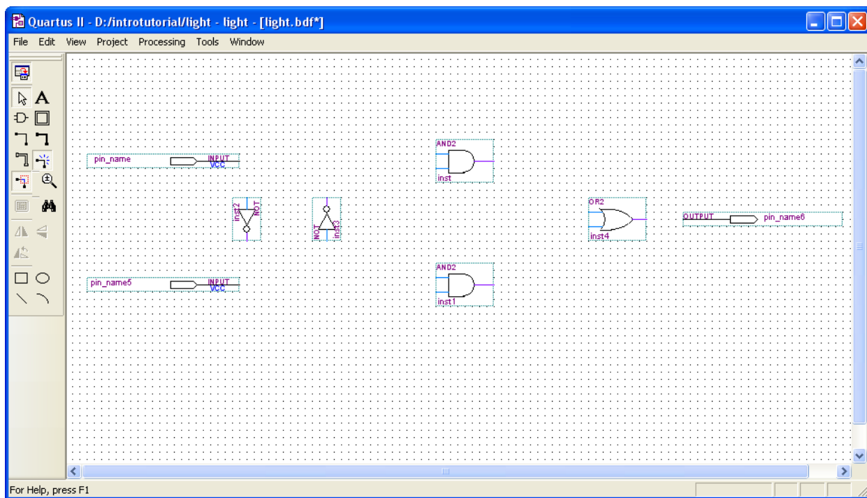
Figure 17. Import the input and output pins.
