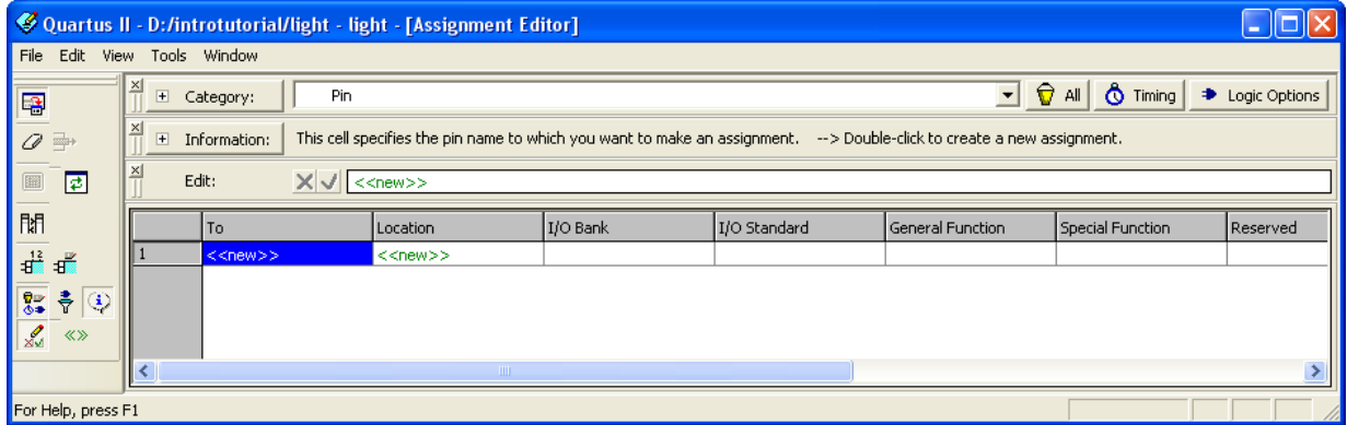
Figure 24. The Assignment Editor window.
