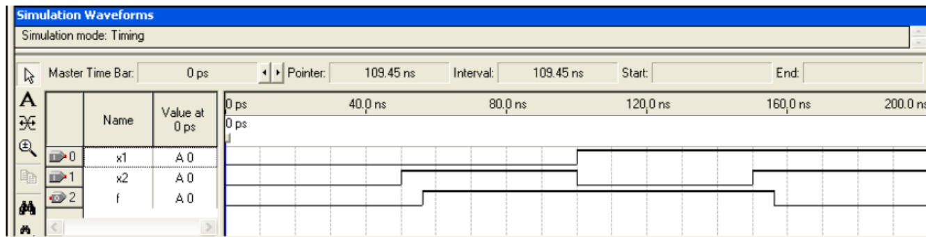
Figure 39. The result of timing simulation.
