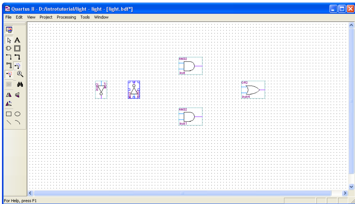
Figure 16. Import the gate symbols into the Graphic Editor window.
