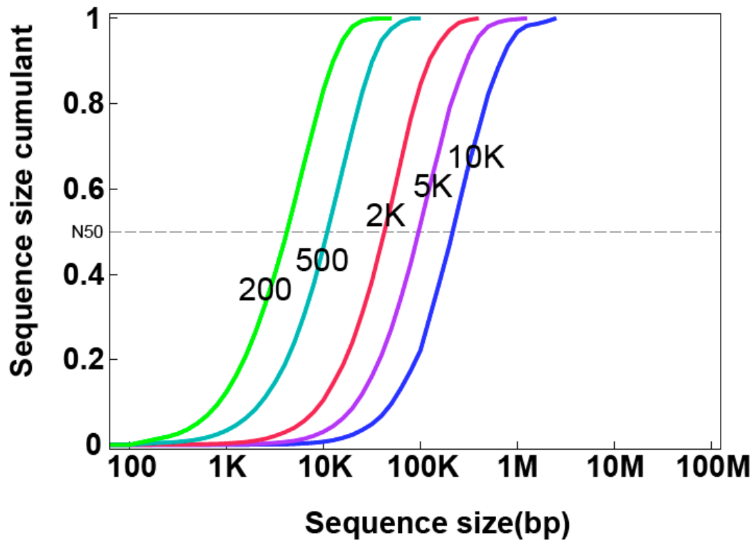
Supplementary figure 9. Sequence length distribution of ideal assembly with each insert-sized paired-ends in the rice genome.
