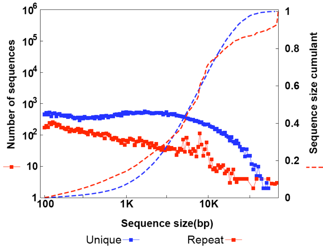
Supplementary figure 4. Length distribution of unique and repeat sequence clusters in the drosophila genome. We used 25-mer.
