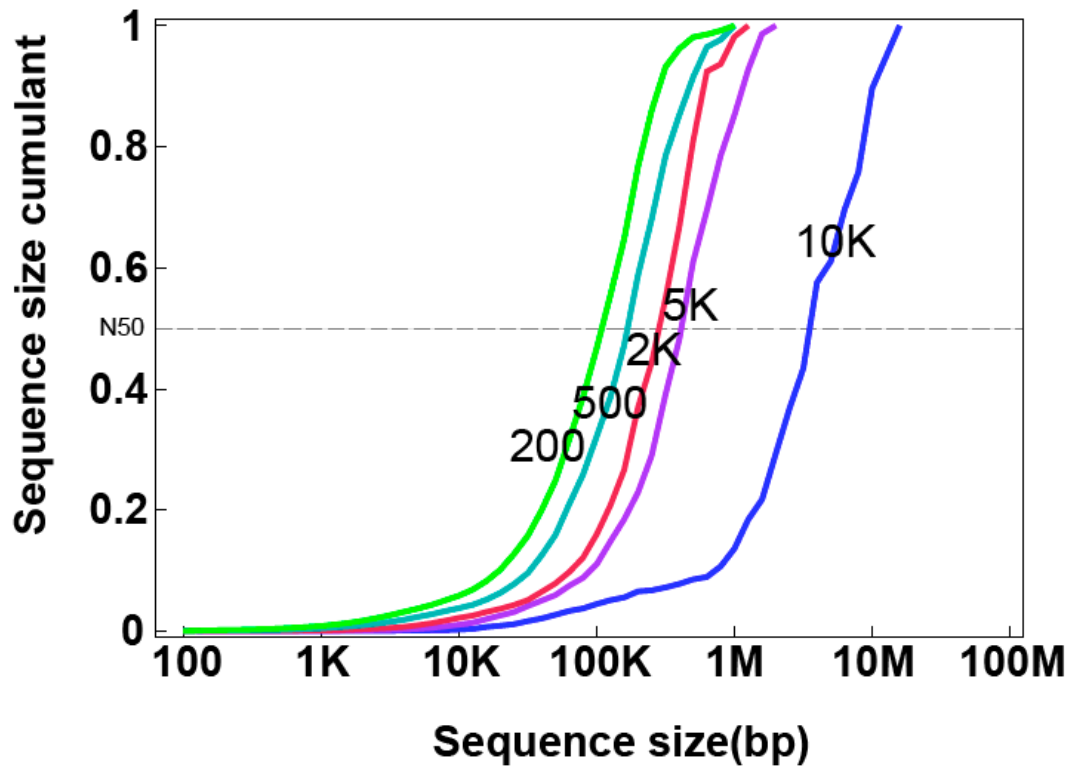
Supplementary figure 7. Sequence length distribution of ideal assembly with each insert-sized paired-ends in the drosophila genome.
