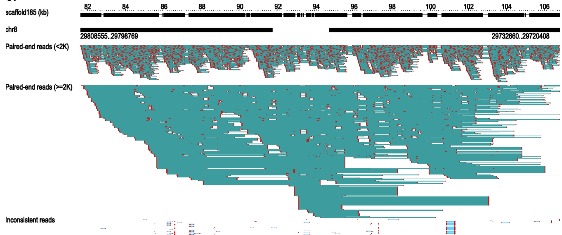
Supplementary figure 3. Cases of structural discrepancy between the assembled scaffolds and the NCBI human reference genome (build 36). The read sequences were displayed in red color, and the clones from which the reads were generated from were drawn in light blue color. A. A case of inversion. B. A case of fragmental substitution. C. A case of deletion.
