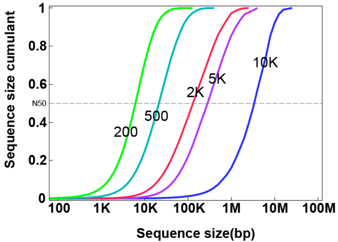
Supplementary figure 8. Sequence length distribution of ideal assembly with each insert-sized paired-ends in the mouse genome.
