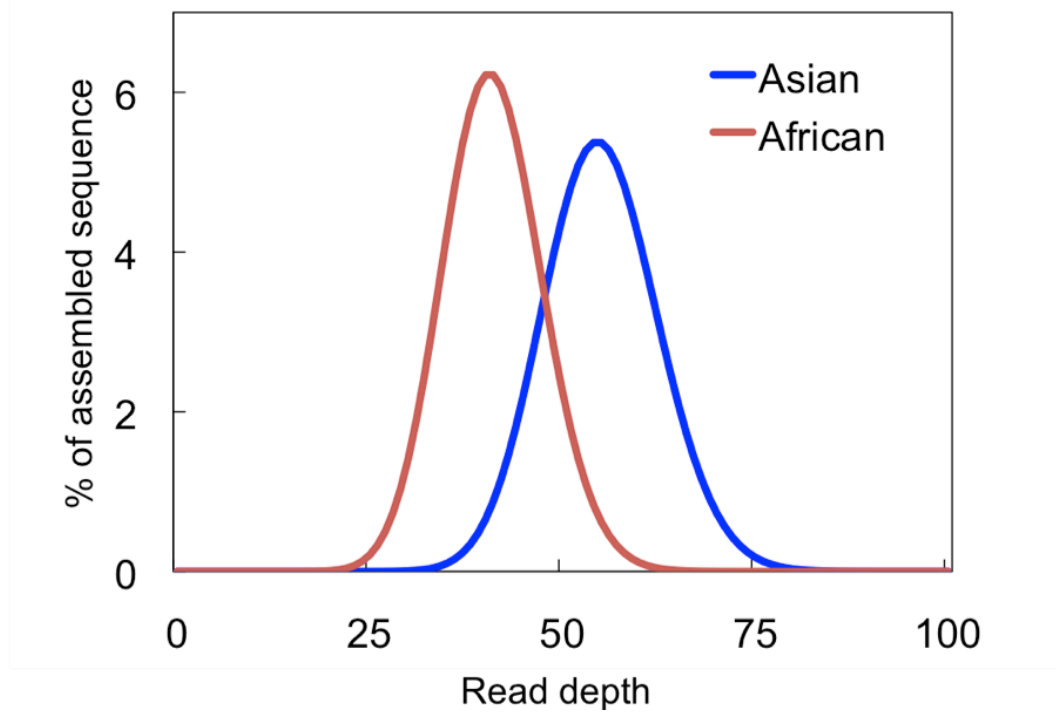
Supplementary figure 2. Distribution of read coverage on the assembled Asian and African genome. The reads were aligned on the genome using SOAP by allowing at most 2 mismatches.
