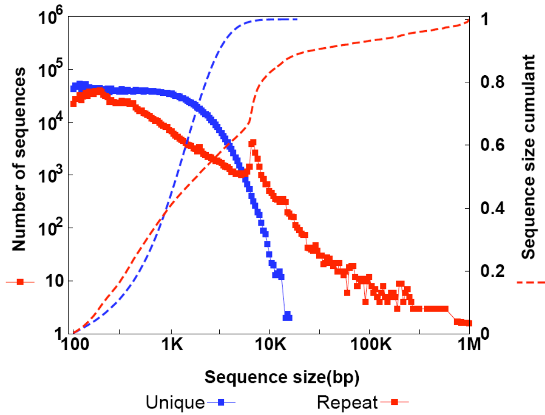
Supplementary figure 5. Length distribution of unique and repeat sequence clusters in the mouse genome. We used 25-mer.
