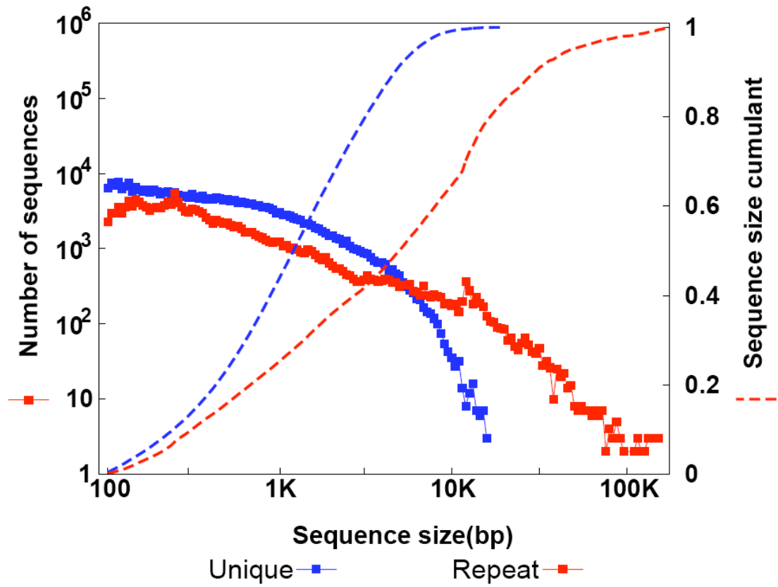
Supplementary figure 6. Length distribution of unique and repeat sequence clusters in the rice genome. We used 25-mer.
