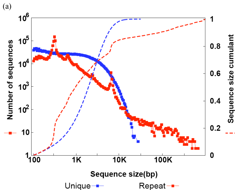
(b) Supplementary figure 1. Length distribution of unique and repeat sequence clusters in the human genome. (a) 21-mer was used; (b) 29-mer was used. Refer to figure 1a.
